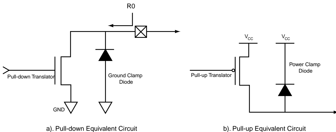
Figure 8 • Pull-down and Pull-up Equivalent Resistors
