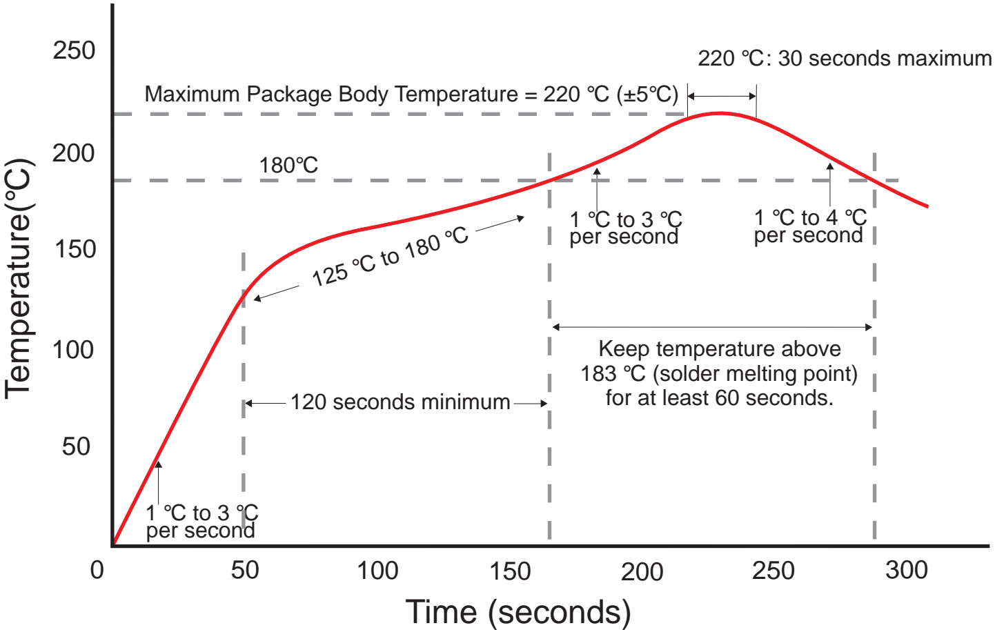
Figure 4 Sample Temperature Profile for I/R or Convection Reflow
