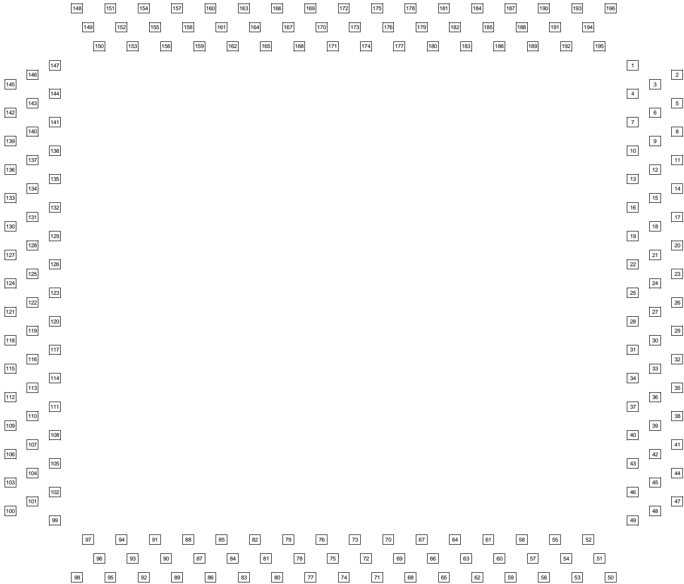
SY-CQ196 Pin Assignment with 196-pin CQFP Top View
