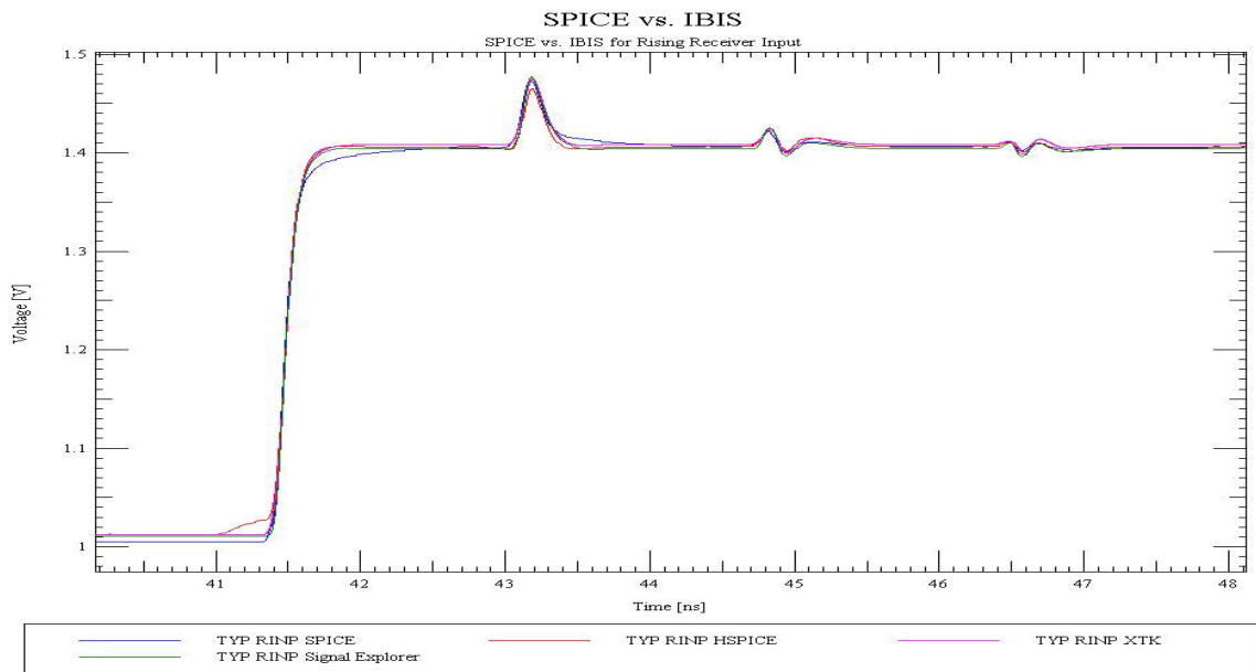
Figure 15. SPICE vs. IBIS for Single-Ended LVDS Receiver Input
