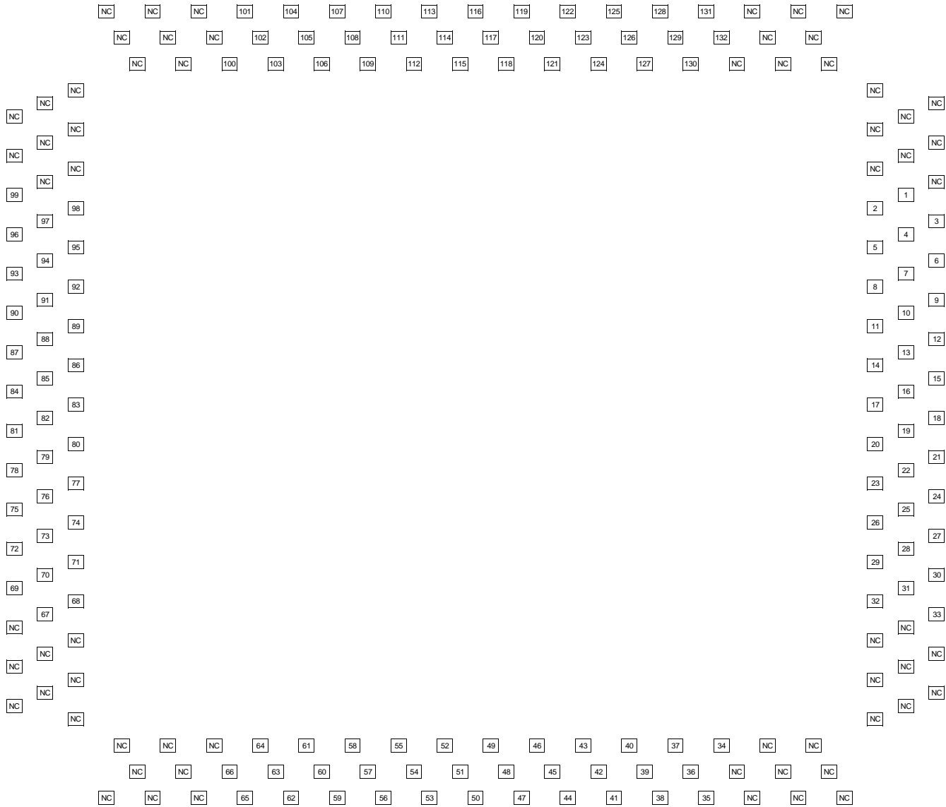
SY-CQ196 Pin Assignment with 132-pin QFP Top View
