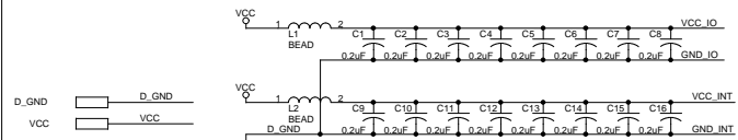
As many as possible Decoupling cap
