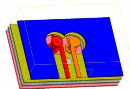
Package build-up layer vias for RocketIO signals
